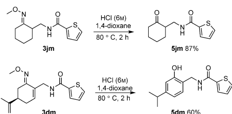
Scheme 6. Deprotection of C(sp 3 )–H amination products.
