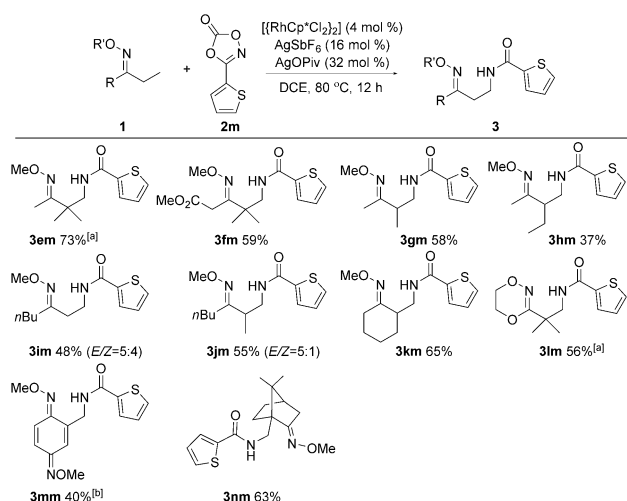
Scheme 4. C–H amidation of other aliphatic O-methyl ketoximes. Reaction conditions: 1 (0.2 mmol), 2m (0.21 mmol), AgOPiv (32 mol %), [\text{RhCp}^*\text{Cl}_2]_2 (4 mol %), AgSbF 6 (16 mol %), DCE (3.0 mL), 80 °C, 12 h, sealed tube under nitrogen. Yield is that of product isolated after column chromatography. [a] Reaction was performed with AgOAc (8 mol %) in CH 2 Cl 2 at 25 °C. [b] Reaction was performed with AgOAc (8 mol %) in CH 2 Cl 2 at 80 °C.
